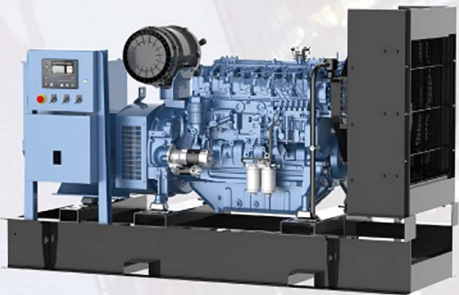
F series base fuel tank type
